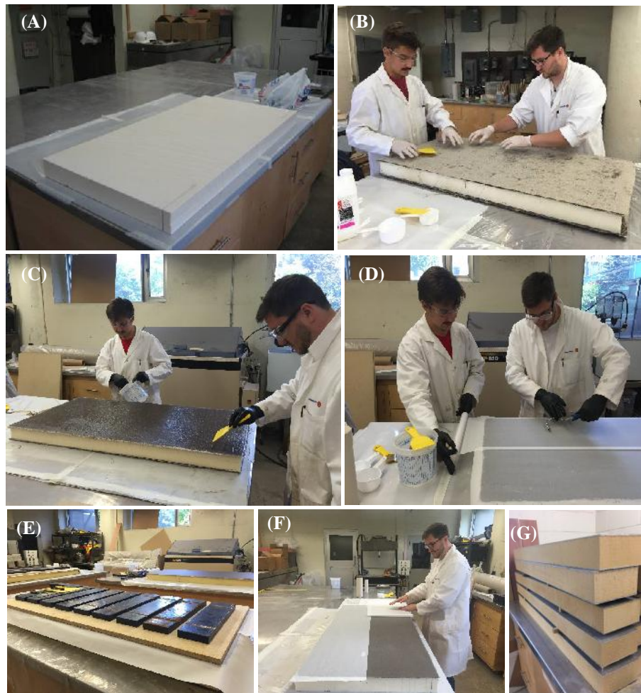
FIGURE 1 – SPECIMEN FABRICATION: (A) PLAIN FOAM SECTION (B) APPLICATION OF FLAX LAYER (C) APPLICATION OF BIO-BASED EPOXY (D) APPLICATION OF PARCHMENT PAPER (E) CURING (F) REMOVAL OF PARCHMENT PAPER (G) FINISHED SAMPLES
