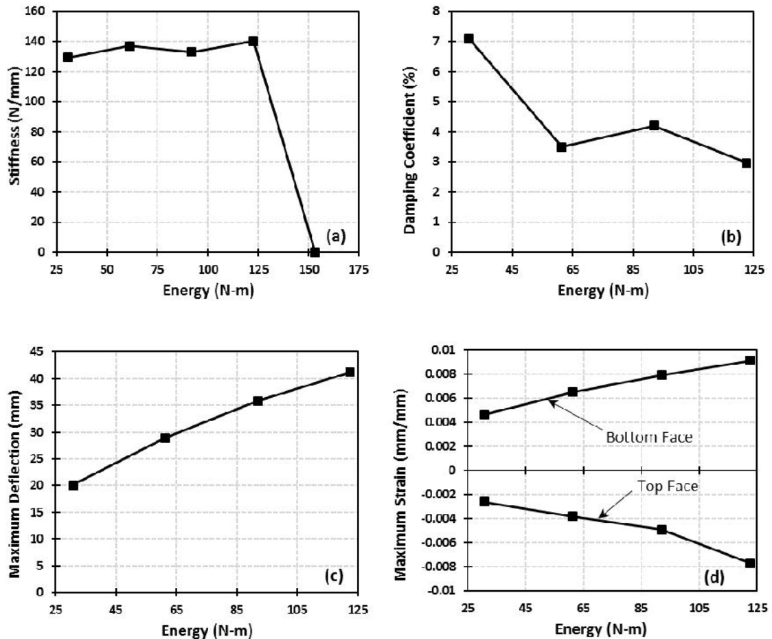
FIGURE 8 – EFFECT OF INPUT ENERGY ON SPECIMEN (A) STIFFNESS (B) DAMPING COEFFICIENT (C) MAXIMUM DISPLACEMENT (D) MAXIMUM FACING STRAIN
