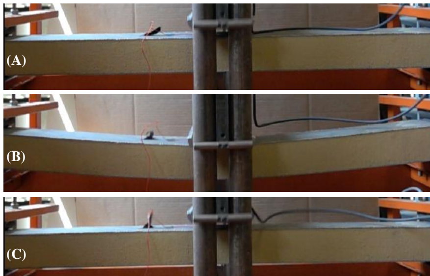
FIGURE 3 – IMPACT EVENT FROM A DROP HEIGHT OF 1200 MM (A) BEFORE IMPACT (B) MAXIMUM DEFLECTION (C) AFTER IMPACT
