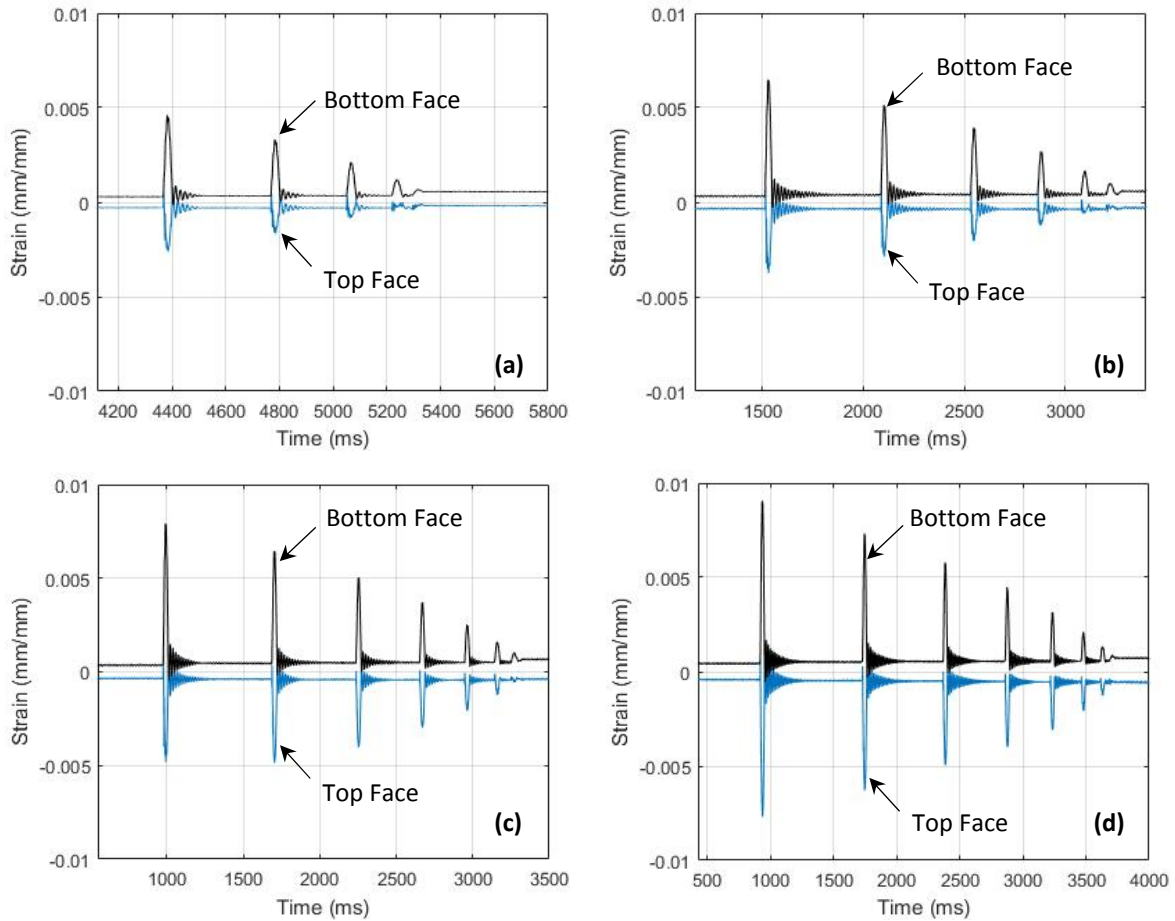
FIGURE 6 – STRAIN VS. TIME (A) 300 MM DROP (B) 600 MM DROP (C) 900 MM DROP (D) 1200 MM DROP
