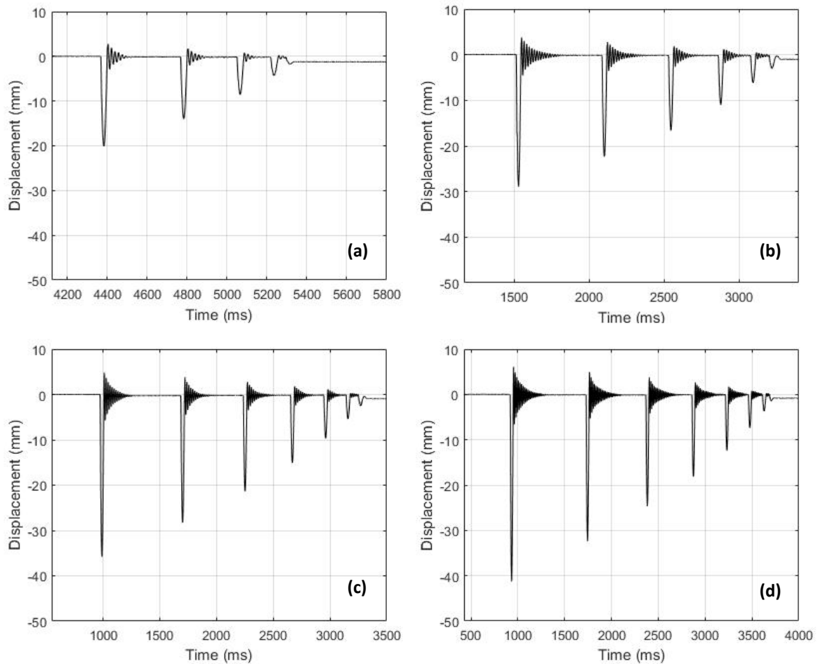
FIGURE 4– DEFLECTION VS. TIME (A) 300 MM DROP (B) 600 MM DROP (C) 900 MM DROP (D) 1200 MM DROP
