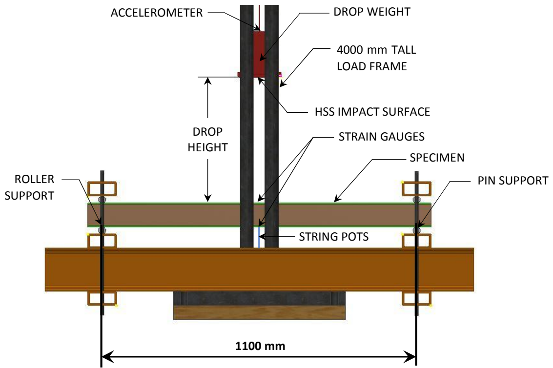
FIGURE 2 – TEST SET-UP
