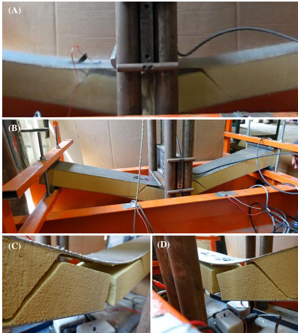
FIGURE 7 – SPECIMEN FAILURE AT DROP HEIGHT OF 1500 MM (A) DURING IMPACT (B) AFTER IMPACT (C) DETAIL (D) DETAIL
