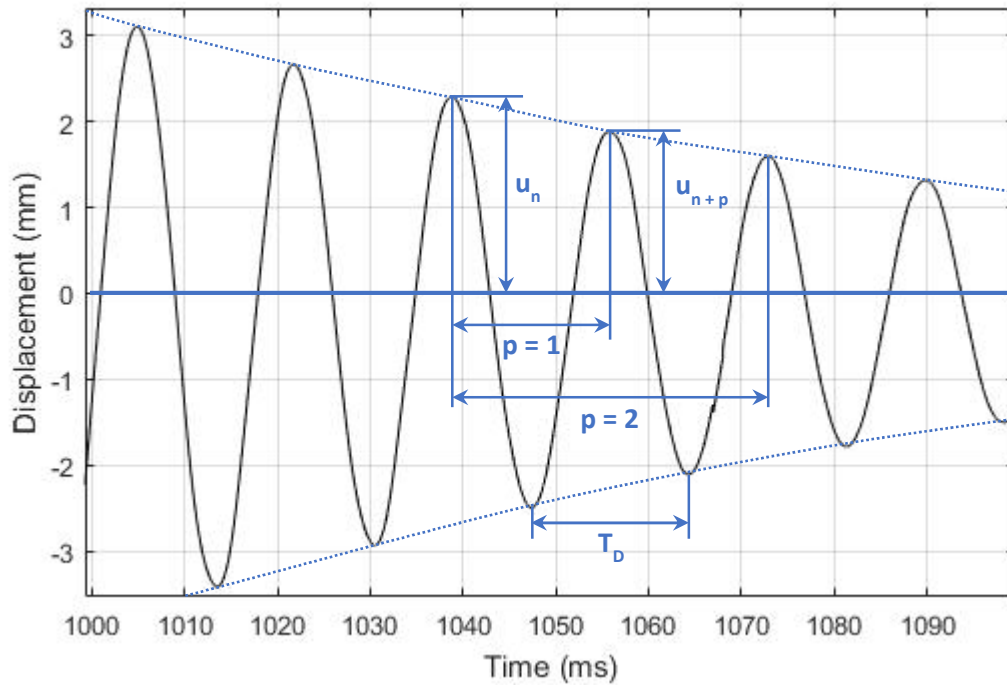
FIGURE 5 – DAMPING OF SANDWICH PANEL UNDER FREE VIBRATION
